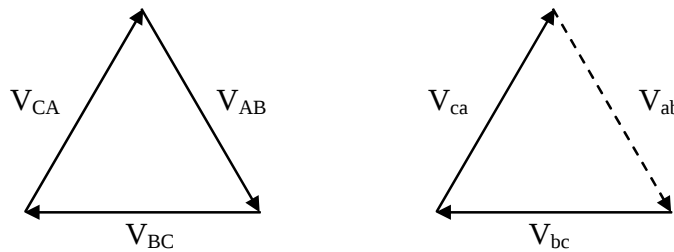
Fig. 6.14 (i) Open delta connection (ii) Phasor diagram for open delta
