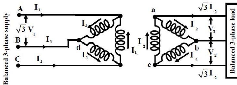
Fig. 6.4 Delta-Delta connections
