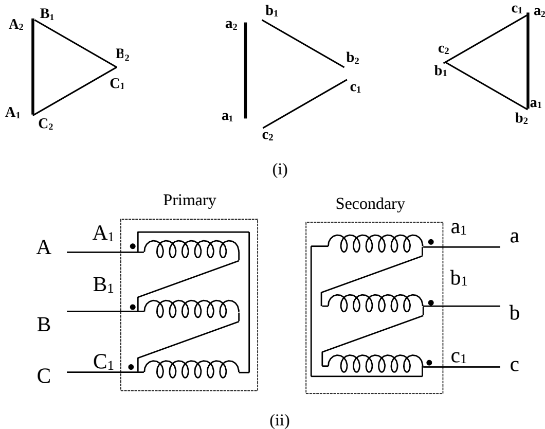
Fig. 6.22 Phasor diagram of Dd6 arrangement (ii) Connection diagram for it
