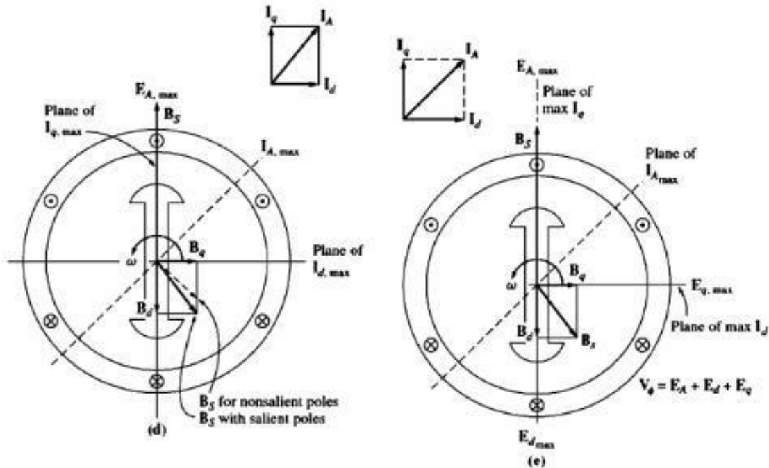
Fig.3.2: The effects of armature reaction in a salient-pole synchronous generator.
