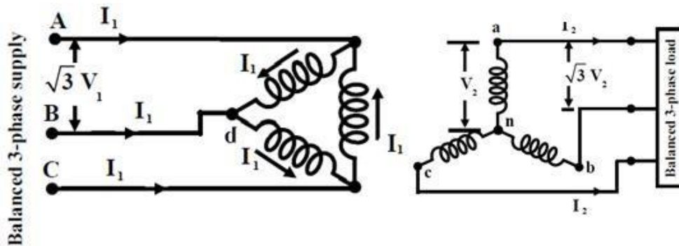
Fig. 6.6 Delta-Star connections
