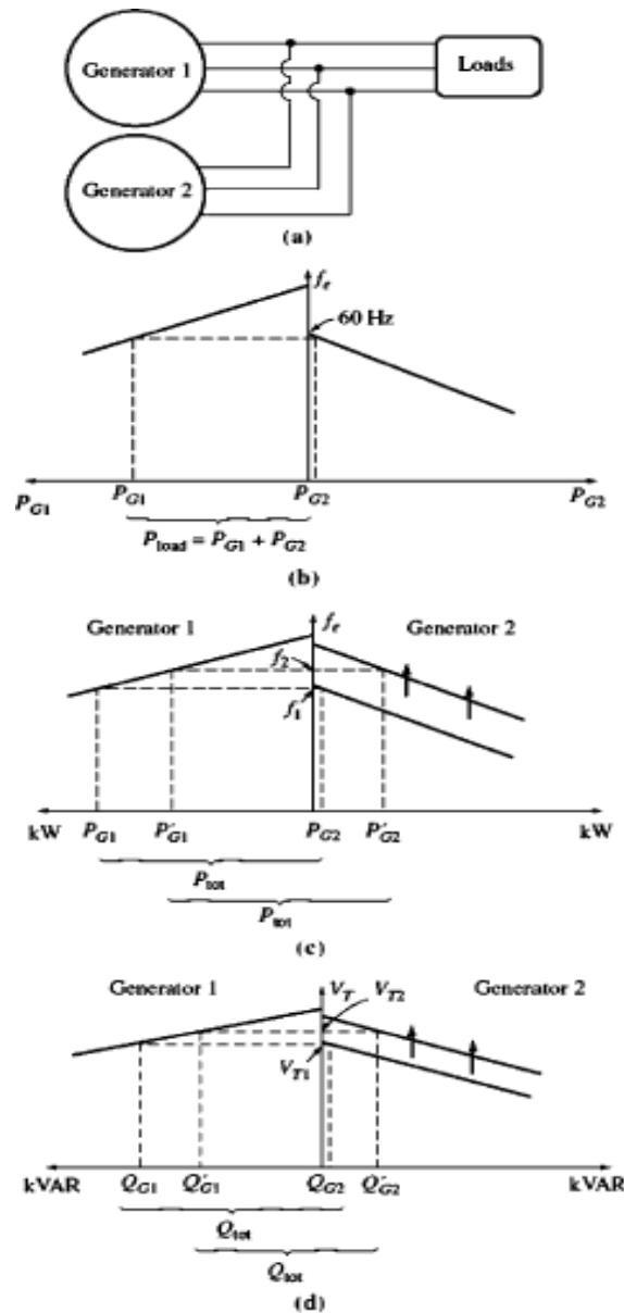
Fig.4.11 (a) A generator Connected in parallel with another machine of the same size. (b) The corresponding house diagram at the moment generator 2 is paralleled with the system.(e) The effect of increasing generator 2's governor set points on the operation of the system.(d) The effect of increasing generator 2's field current on the operation of the system.
