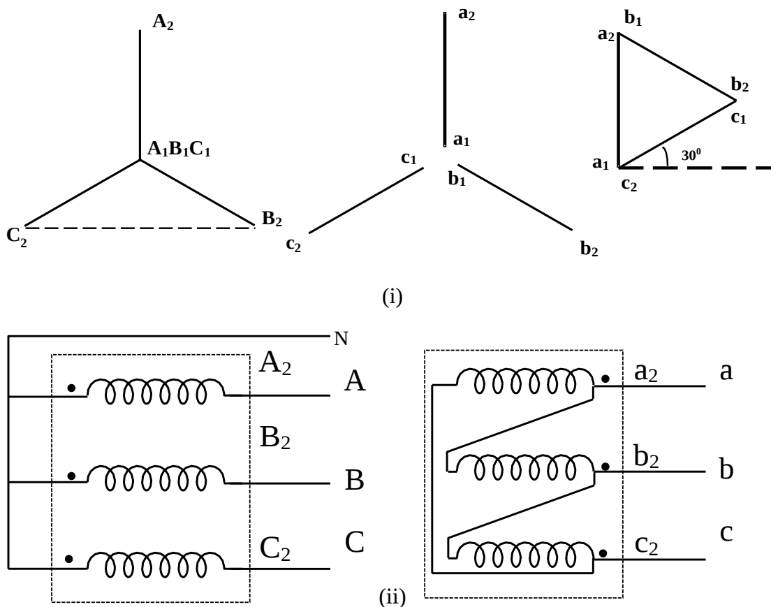
Fig. 6.27 Phasor diagram of Yd11 arrangement (ii) Connection diagram for it
