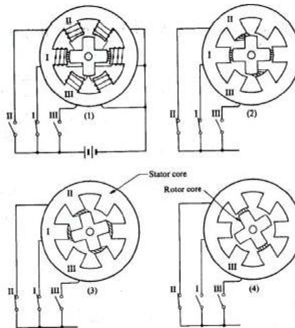
Fig. 7.15: Stepper motor states for motion
