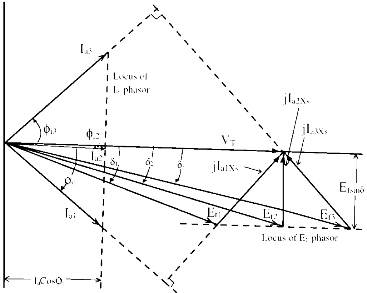
Fig. 5.7: Phasor diagram showing effect of changes in field excitation on armature current, power angle and power factor of a synchronous motor
