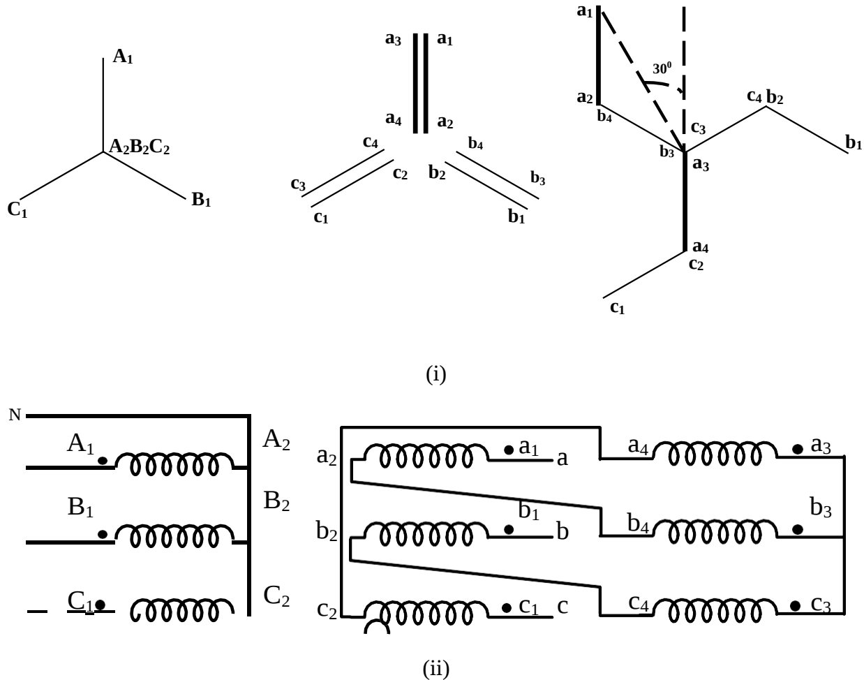
Fig. 6.29 Phasor diagram of Y11 arrangement (ii) Connection diagram for it
