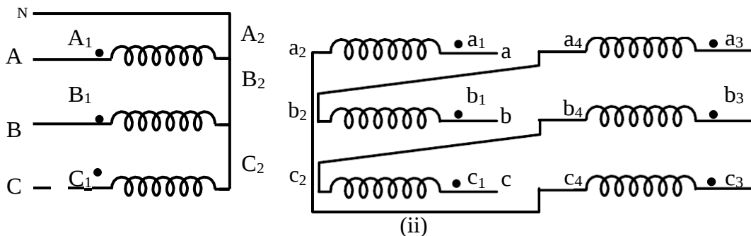
Fig. 6.26 Phasor diagram of Yz1 arrangement (ii) Connection diagram for it
