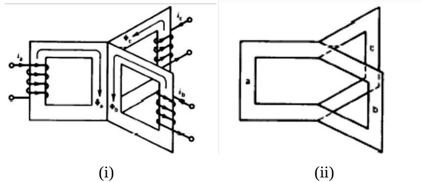
Fig. 6.1 Three phase core type transformer
