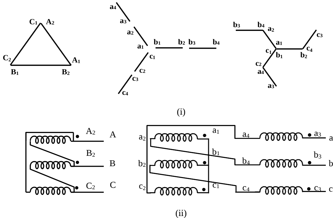
Fig. 6.23 Phasor diagram of Dz6 arrangement (ii) Connection diagram for it
